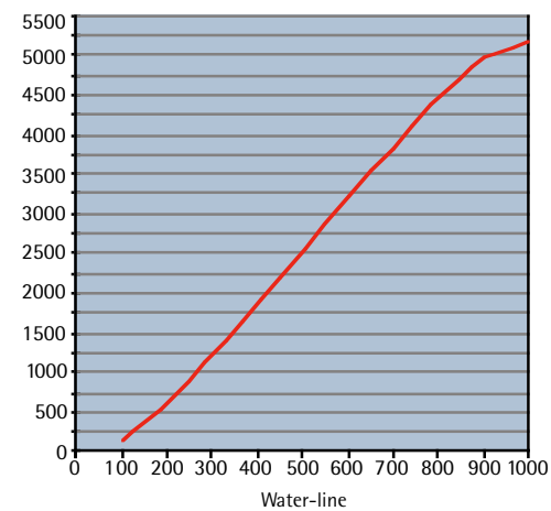
BUOYANCY DIAGRAM
